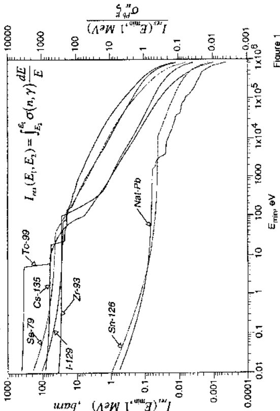
Figure 74: resonance integral for elements produced in reactors. A sudden drop in I_{res} indicates a resonant capture at a particular neutron energy.
