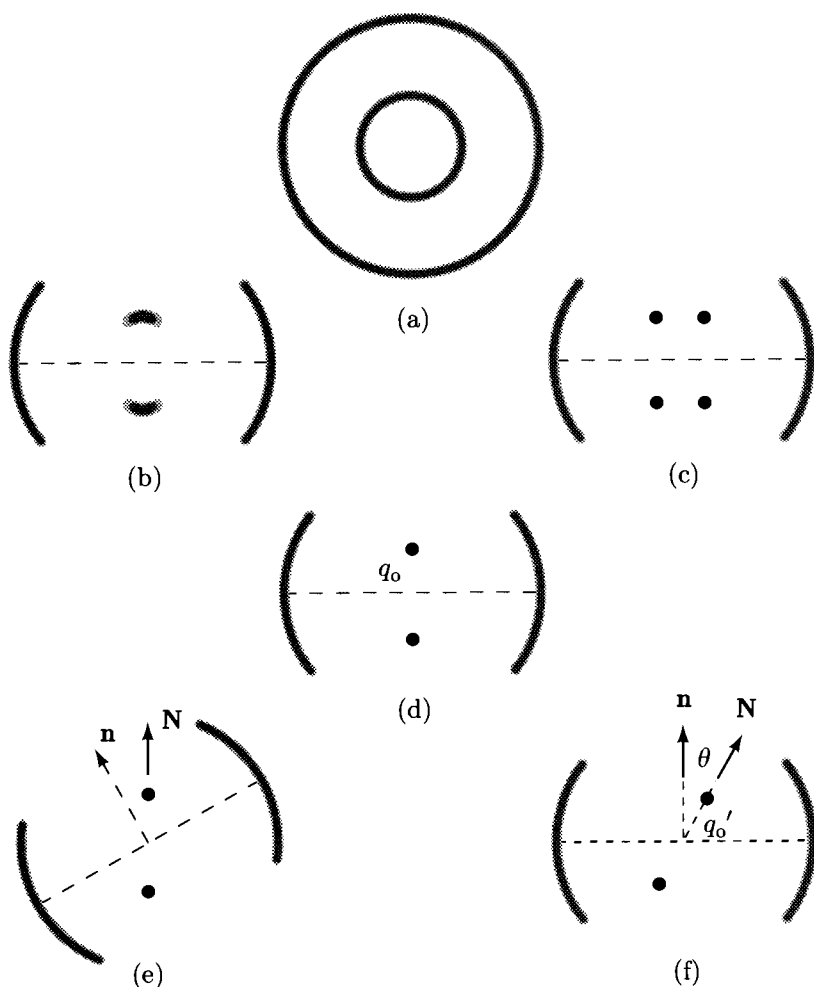
Fig. 2.7.4. Schematic representation of X-ray scattering intensities profiles from (a) the isotropic, (b) and (c) the nematic, (d) the smectic-A, and (e) and (f) the smectic-C phases. All intensities profiles are cross-sections in a plane containing the director \mathbf{n} . The full three-dimensional profiles for (a) through (d) are obtained by rotating the cross-sectional profiles about \mathbf{n} . (b) and (c) apply, respectively, to nematic phases near transitions to the smectic-A and smectic-C phases. The former has diffuse spots at \mathbf{q} = \pm q_0 \mathbf{n} whereas the latter has diffuse rings in the plane perpendicular to \mathbf{n} very nearly centered at \mathbf{q} = \pm (2\pi/l) \mathbf{n} . The smectic-A phase has quasi-Bragg peaks at \mathbf{q} = \pm q_0 \mathbf{n} , and the smectic-C phase has peaks at \mathbf{q} = \pm q'_0 \mathbf{N} where q'_0 is very nearly 2\pi/(l \cos \theta) where \theta is the angle between \mathbf{N} and \mathbf{n} . (e) and (f) are identical except for alignment of axes. The full three-dimensional scattering profile for the smectic-C phase is not invariant with respect to rotations about \mathbf{n} .
