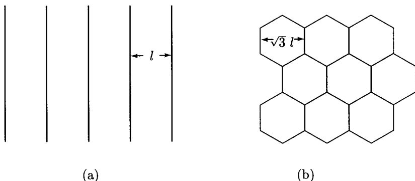
Fig. 10.3.7. (a) A striped incommensurate phase consisting of a linear array of equally spaced domain walls. (b) A hexagonal incommensurate phase in which domain walls follow the edges of a honeycomb lattice.
