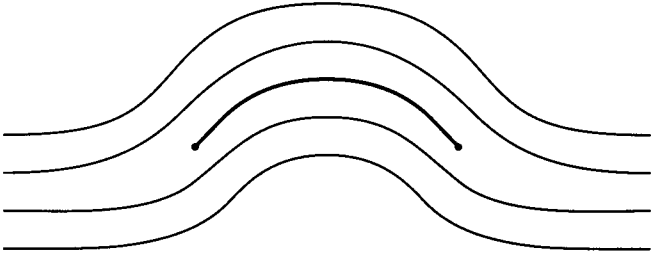
Fig. 9.2.8. An edge dislocation loop with a distorted covering surface.
