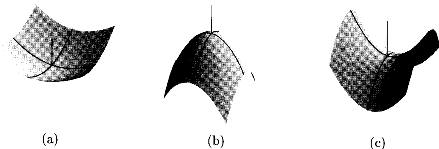
Fig. 10.4.4. Sections of surfaces (a) with two positive radii of curvature, (b) with two negative radii of curvature, and (c) with one positive and one negative radius of curvature. The surface in (a) has positive mean and Gaussian curvature at P ; that in (b) has negative mean and positive Gaussian curvature; and that in (c) has negative Gaussian curvature and mean curvature whose sign depends on the relative magnitude of R_1 and R_2 .
