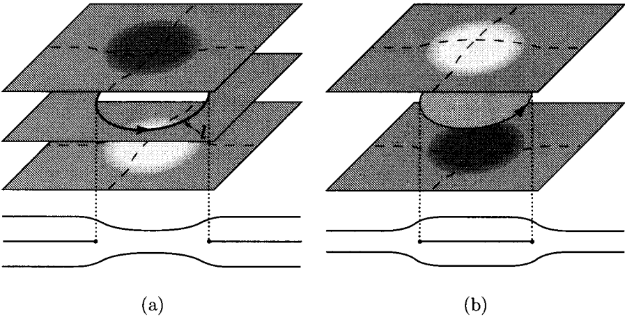
Fig. 9.2.7. Edge dislocation loops. (a) A +d loop corresponding to removal of matter from interior of loop. (b) A -d loop corresponding to insertion of a layer inside loop.
