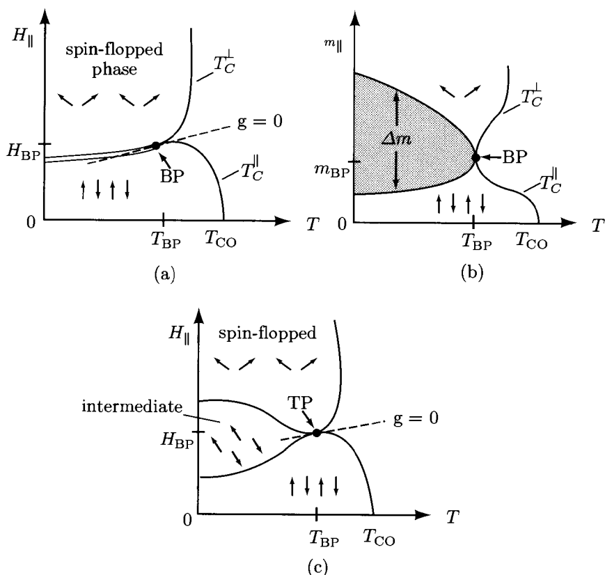
Fig. 4.6.11. (a) Schematic representation of a phase diagram of an anisotropic antiferromagnet in a field with a spin-flop bicroritical point (BP). In the antiferromagnetic phase, the average spin in each of the two sublattices is either parallel or antiparallel to the anisotropy axis for H_{BP} > H > 0 . The magnitude of the spin is greater in one sublattice than in the other. In the spin-flop phase, the component of the spin parallel to the field is the same in both sublattices, and the component perpendicular to the field alternates in sign. (b) Same as (a) but in the m - T plane. (c) Schematic representation of a phase diagram for an anisotropic antiferromagnet with a tetracritical point (TP). [Michael E. Fisher and David R. Nelson, Phys. Rev. Lett. 32 , 1350 (1974).]
