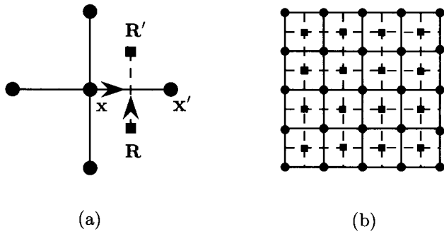
Fig. 9B.2. (a) This figure shows the construction of the nearest neighbor bond \langle \mathbf{R}, \mathbf{R}' \rangle in the dual lattice \mathcal{L}_{\square}^D from its associated bond \langle \mathbf{x}, \mathbf{x}' \rangle in the lattice \mathcal{L}_{\square} . A direction pointing from the site \mathbf{x} to the site \mathbf{x}' is assigned to the bond \langle \mathbf{x}, \mathbf{x}' \rangle . The bond \langle \mathbf{R}, \mathbf{R}' \rangle is the perpendicular bisector \langle \mathbf{x}, \mathbf{x}' \rangle and points in a direction determined by the right hand rule relative to the normal pointing out of the page. (b) A section of the lattice \mathcal{L}_{\square} and its associated dual lattice \mathcal{L}_{\square}^D . Sites and bonds in \mathcal{L}_{\square} are, respectively, represented as full circles and solid lines; those in \mathcal{L}_{\square}^D are shown as squares and dashed lines.
