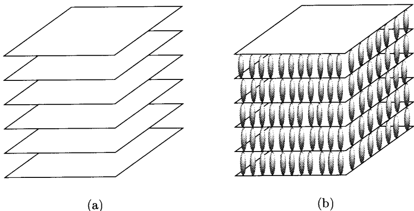
Fig. 6.3.1. (a) Parallel planes of a layered structure. (b) Planes interpreted as separating successive planes of molecules.
