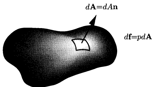
Fig. 3.1.1. A fluid contained in a volume element exerts an outward force normal to its surface. The force d\mathbf{f} exerted on an element of area dA = dA\mathbf{n} with unit normal \mathbf{n} is parallel to \mathbf{n} and proportional to dA : d\mathbf{f} = p d\mathbf{A} . p is the pressure with units of force per unit area or energy per unit volume.
