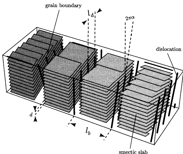
Fig. 9.6.1. Schematic representation of the TGB phase. There are smectic slabs with layer spacing d and length l_b . Between each pair of smectic slabs is a twist-grain boundary consisting of parallel screw dislocations separated by a distance l_d . The angle between dislocation cores in adjacent grain boundaries or, equivalently, between layer normals in adjacent smectic slabs is 2\pi\alpha = \delta\theta = 2 \tan^{-1}(d/2l_d) . If \alpha is irrational, then no two slabs have identical layer normals, and there is an incommensurate TGB phase. If \alpha = P/Q (with P and Q relatively prime integers) is a rational number, then there is a quasicrystalline TGB phase.
