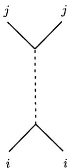
Fig. 5B.5. Representation of \overline{\mathcal{H}}_\Lambda^4 for O_n models. The dashed line represents the vertex u . At each end of this vertex are a pair of \phi lines with the same Cartesian index i or j = 1, \dots, n .
