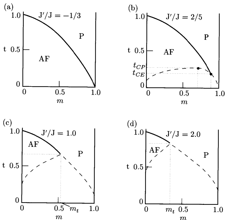
Fig. 4.6.6. Mean-field phase diagrams for the metamagnet. Here, J = z_1 J_1 and J' = z_2 J_2 . (a) shows only a second-order P-AF transition. (b) shows a critical endpoint at t_{CE} where the second-order P-AF line meets the first-order coexistence line and a critical point at t_{CP} where two-phase coexistence ends. (c) and (d) show second-order P-AF lines terminating at a tricritical point. [J.M. Kincaid and E.G.D. Cohen, Phys. Rep. C 22 , 57 (1975).]
