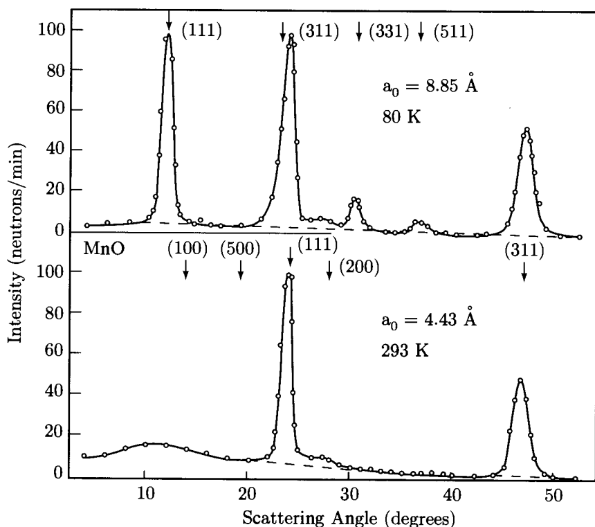
Fig. 2.11.3. Neutron diffraction patterns for MnO below and above the spin ordering temperature of 120K (see Fig. 2.11.2d). The reflection indices are based on an 8.85\text{\AA} cell at 80K and a 4.43\text{\AA} cell at 293K. [C.G. Shull, W.S. Strauser, and E.O. Wollan, Phys. Rev. 83 , 333 (1951). G.G. Low, Application of neutron scattering to magnetism, in Magnetism, "Selected Topics" , ed. S. Foner (Gordon and Breach, NY, 1976).]
