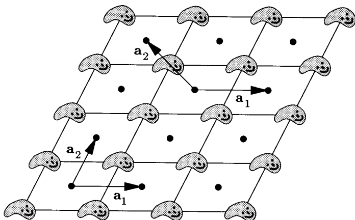
Fig. 2.5.1. A two-dimensional crystal consisting of identical unit cells periodically repeated to fill space. Two sets of primitive translation vectors are shown.
