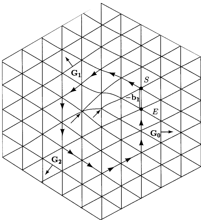
Fig. 9.2.15. A dislocation in a two-dimensional hexagonal crystal. The lines in this figure are lines of constant phase of the three mass-density waves of the crystal. The Burgers vector is -b_1 , and extra lines are inserted from the right in the grids perpendicular to G_1 and G_2 . The Burgers circuit around the core starts at S and ends at E . The vector connecting S to E is the vector -b_1 shown in Fig. 9.2.14. Note that, in the core region, there is a site with five neighbors and a site with seven neighbors, indicating that a dislocation can be viewed as a disclination pair.
