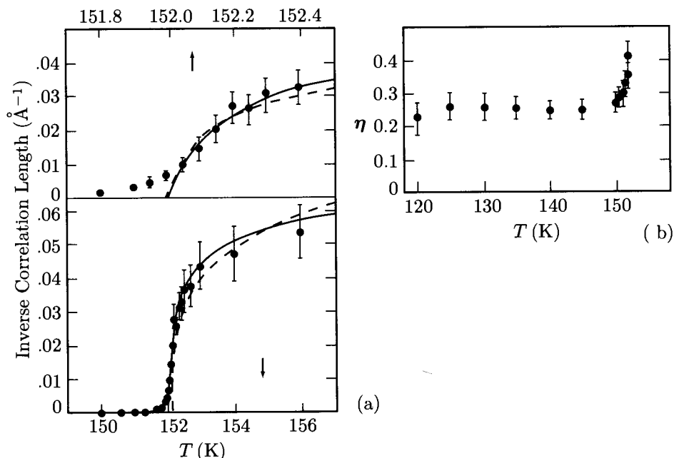
Fig. 6.4.5. (a) Inverse scattering lengths from Lorentzian fits to the structure function. Solid lines are fits to the dislocation mediated melting theory (see Chapter 9). Top and bottom panels are the same fits with different scales. (b) \eta = \eta_{G=(1,0)} for the solid phase of Xe on graphite. [P. A. Heiney, P. W. Stephens, R. J. Birgeneau, P. M. Horn, and D. E. Moncton, Phys. Rev. B 28 , 6416 (1983).]
