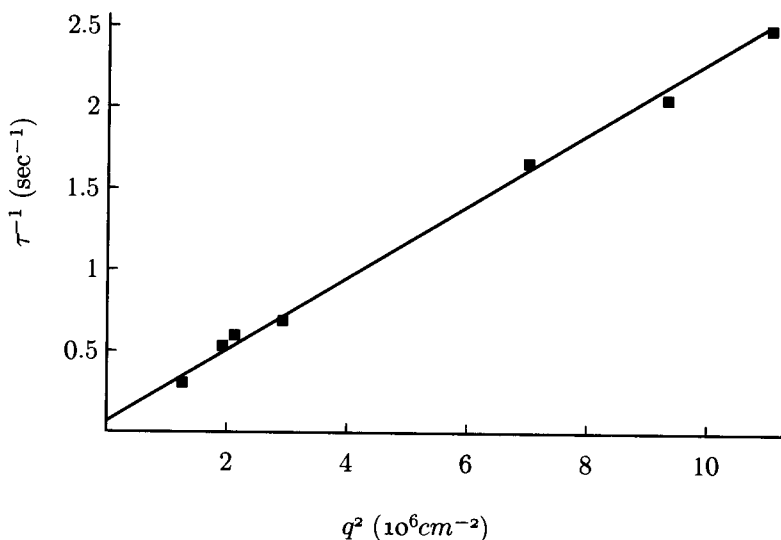
Fig. 7.4.4. Inverse decay time as a function of q^2 for self-diffusion measured by forced Rayleigh scattering. [Courtesy of W.D. Dozier.]
