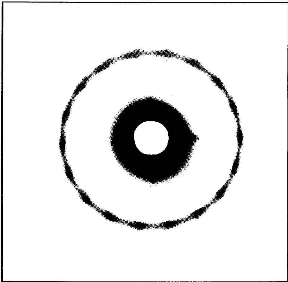
Fig. 9.6.5. Experimental scattering intensity from a quasicrystalline TGB phase showing 18 Bragg peaks around a ring. This material is a \text{TGB}_C phase, in which the smectic slabs are smectic-C slabs in which the director is not parallel to the layer normal. It has either 9- or 18-fold quasicrystalline symmetry. [L. Navailles, P. Barrios, and H. Nguyen, Phys. Rev. Lett. 71 , 545 (1993).]
