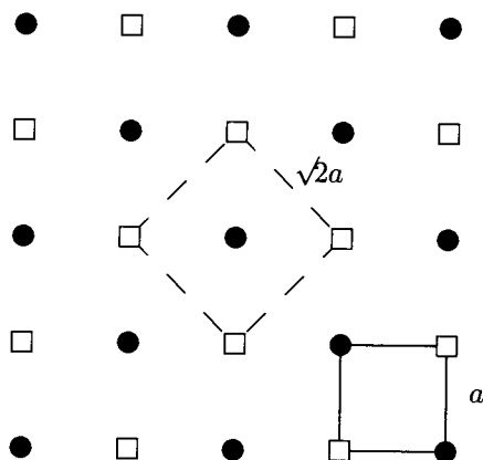
Fig. 5.7.1. An Ising model on a square lattice showing the original lattice with N sites (marked • and □) and lattice constant a and the new lattice with N' = b^{-2}N sites and lattice constant ba = \sqrt{2}a after spins at the sites marked by • have been removed by decimation. Also indicated are a plaquette of the new (dashed lines) and one of the original (solid lines) lattices. Four-spin interactions involve products of spins on a plaquette.
