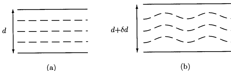
Fig. 6.3.5. Buckling instability of a smectic. (a) Equilibrium configuration and (b) stretched configuration showing undulations.
