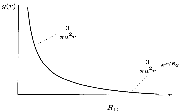
Fig. 2.12.1. Schematic sketch of g(r) for a random-walk polymer chain showing the self-similar behavior for r < R_G .
