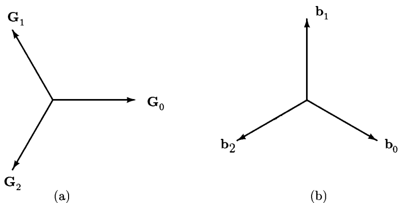
Fig. 9.2.14. (a) The vectors \mathbf{G}_0 , \mathbf{G}_1 and \mathbf{G}_2 in a hexagonal reciprocal lattice. (b) Vectors \mathbf{b}_0 , \mathbf{b}_1 and \mathbf{b}_2 in the direct lattice. The vectors \mathbf{b}_0 and \mathbf{b}_1 form a basis for the direct lattice and satisfy \mathbf{b}_i \cdot \mathbf{G}_j = 2\pi\delta_{ij} .
