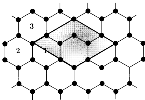
Fig. 5.7.7. Division of the triangular lattice of hexagonal adsorption sites into a superlattice of cells each containing three sites. A unit cell of the superlattice is shaded.
