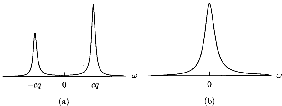
Fig. 8.2.2. (a) S_{\theta\theta}(\mathbf{q}, \omega) and (b) S_{ee}(\mathbf{q}, \omega) for fixed q . Note that the thermal factor in S_{\theta\theta} causes the peak at -cq to have a lower intensity for T > 0 than the peak at +cq . Both the diffusive and propagating peaks have widths proportional to q^2 .
