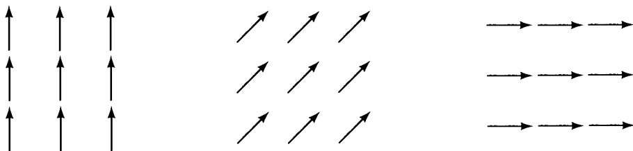
Fig. 6.1.1. Different ground states for the xy -Hamiltonian. The vector order parameter can point anywhere in a two-dimensional plane.
