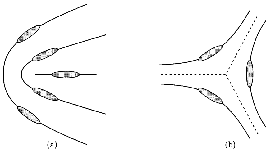
Fig. 9.2.25. (a) k = 1/2 and (b) k = -1/2 disclinations in a two-dimensional nematic.
