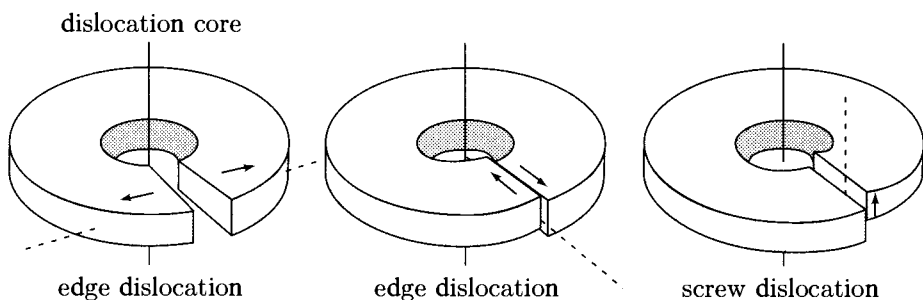
Fig. 9.2.13. The Volterra construction for edge and screw dislocations.
