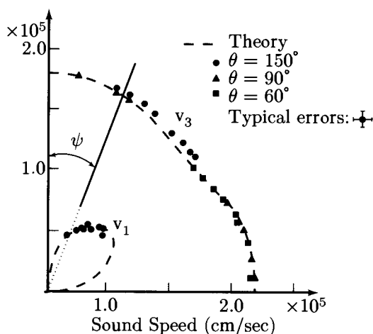
Fig. 8.5.1. Brillouin scattering measurements of the sound velocities in a smectic-A liquid crystal as a function of angle \psi between the wave vector \mathbf{q} and the director \mathbf{n}_0 . v_3 is the velocity of longitudinal sound and v_1 that of transverse sound. It is clear that v_1 is a maximum at \psi = 45^\circ . The experiments are unable to resolve the transverse sound velocity near \psi = 0^\circ and \psi = 90^\circ . v_1 and v_3 , however, lie on the curves predicted by the hydrodynamical theory (see Problem 8.4). The depression in the longitudinal sound velocity at \psi = 45^\circ results from a coupling between longitudinal and transverse sound not present in isotropic fluids. [York Liao, Noel A. Clark, and Peter Pershan, Phys. Rev. Lett. 30 , 639 (1973).]
