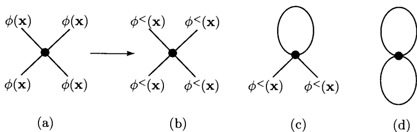
Fig. 5B.1. Diagrams in coordinate space to first order in u . The vertex u is represented by a dot. (a) Representation of the perturbation Hamiltonian \overline{\mathcal{H}}_{\Lambda}^4 before averaging over \phi^> . The four lines represent fields \phi(\mathbf{x}) . Integrating over the fields \phi^> leads to contraction of internal lines and diagrams (b) - (d).
