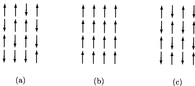
Fig. 3.6.1. Phases for an Ising magnet with Z_2 symmetry. Spins are constrained by crystal fields to point either up or down. (a) Disordered paramagnet, (b) ordered ferromagnet with spins aligned along a common direction, and (c) ordered antiferromagnet on a bipartite square lattice.
