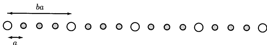
Fig. 5.6.1. Schematic representation of the one-dimensional Ising model showing sites of the original lattice with lattice constant a and sites on the new lattice with lattice constant ba . The b - 1 spins between sites of the new lattice are removed by a trace or decimation operation.
