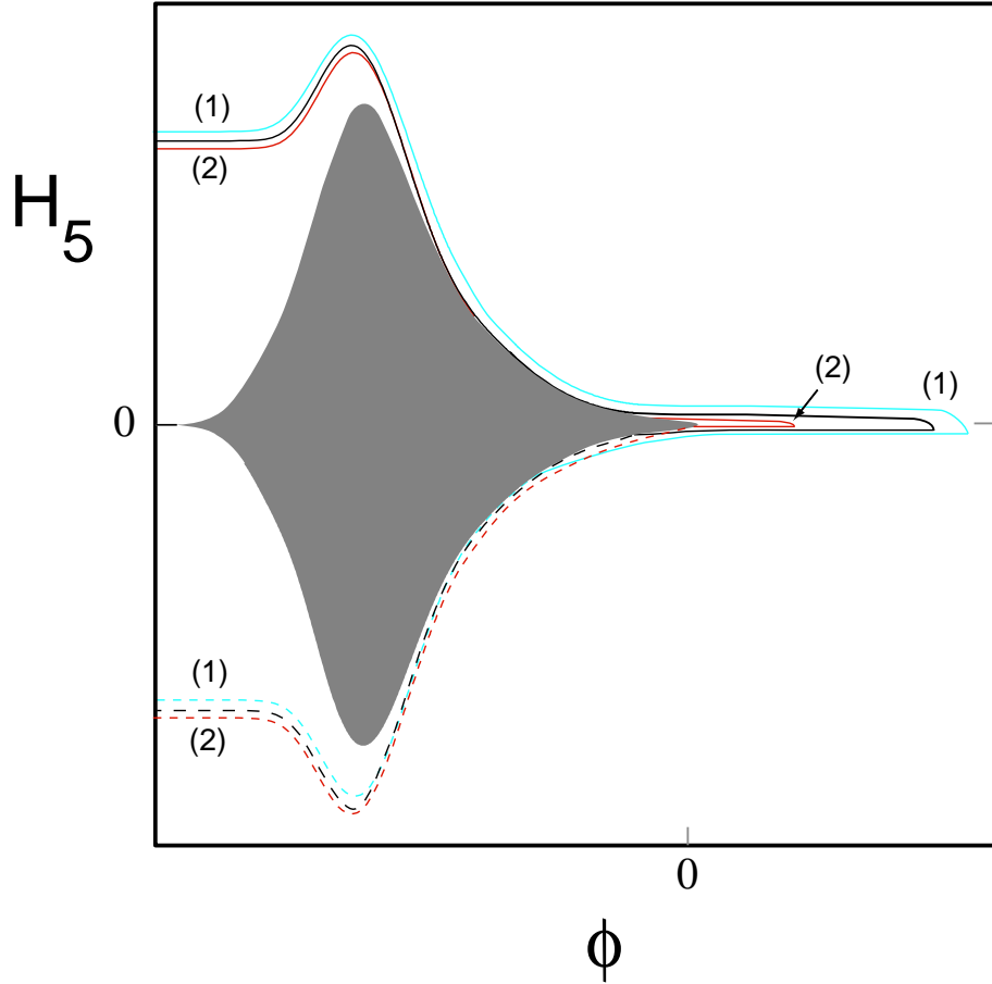
Figure 6: Trajectories in the (H_5, \phi) -plane showing the attractor nature of the cyclic solution (the middle trajectory). Path (1) is an overshoot solution that begins with slightly greater velocity ( H_5 ) than the attractor, bounces off the grey zero-energy surface, and then has a contracting trajectory whose value of H_5 is smaller in magnitude. Path (2) is an undershoot solution which begins with slightly less velocity in the expanding phase than the cyclic value and ends in a contracting phase with H_5 having a slightly greater magnitude. Following the next bounce, therefore, overshoot turns into undershoot and vice-versa. In either case, the deviation from the attractor value shrinks.
