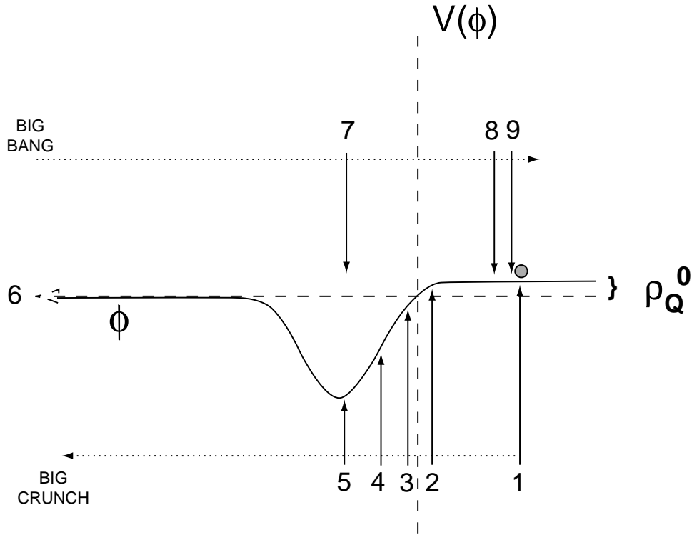
Figure 1: The interbrane potential V(\phi) versus \phi , whose value ( -\infty < \phi < \phi_\infty ) determines the distance between branes. The shaded circle represents the maximum positive value of \phi during the cycle. The various stages are: (1) quintessence/potential domination and cosmic acceleration (duration \geq trillion years); (2) \phi kinetic energy becomes non-negligible, decelerated expansion begins (duration \sim 1 billion years); (3) H = 0 , contraction begins; (4) density fluctuations on observed scales created ( (t_0 t_R)^{1/2} \approx 1 ms before big crunch); (5) \phi kinetic energy domination begins ( t_{min} \sim 10^{-30} s before big crunch); (6) bounce and reversal from big crunch to big bang; (7) end of \phi kinetic energy domination, potential also contributes ( t_{min} \sim 10^{-30} s after big bang); (8) radiation dominated epoch begins t_R \sim 10^{-25} s after big bang); (9) matter domination epoch begins ( \sim 10^{10} s after big bang). As the potential begins to dominate and the Universe returns to stage (1), the field turns around and rolls back towards -\infty .
