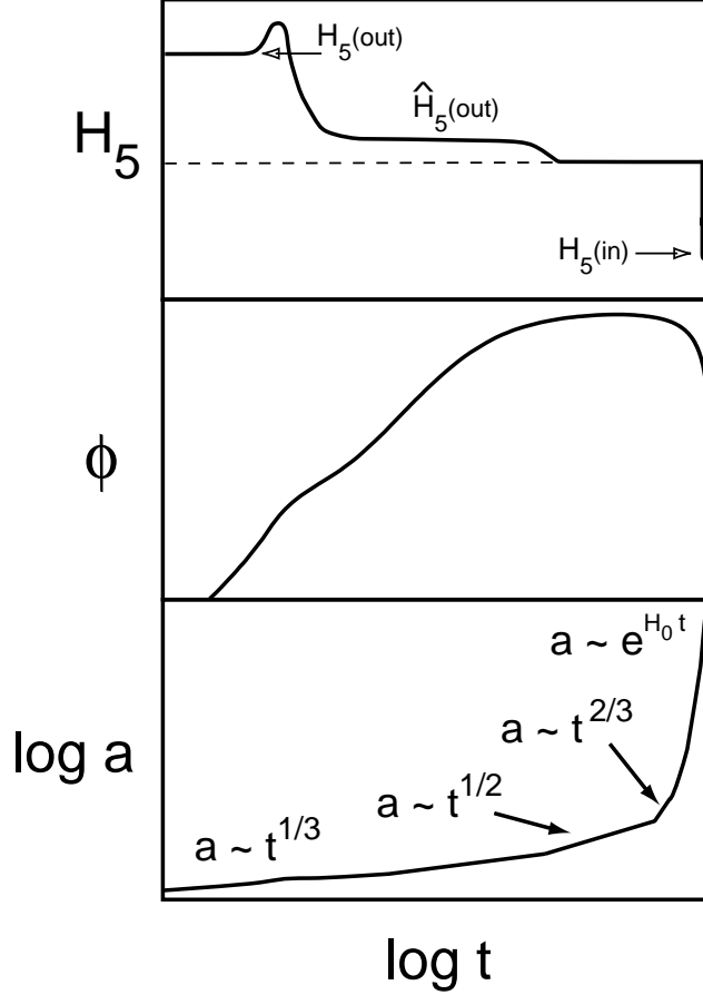
Figure 2: Schematic plot of the scale factor a(t) , the modulus \phi(t) , and H_5 \equiv \frac{2}{3}d(\exp(\sqrt{3/2}\phi))/dt for one cycle, where t is Einstein frame proper time. The scale factor starts out zero but expands as t^{\frac{1}{3}} , and the scalar field grows logarithmically with t , in the scalar kinetic energy dominated early regime. Then, when radiation begins to dominate we have a \propto t^{\frac{1}{2}} , and the scalar field motion is strongly damped. This is followed by the matter era, where a \propto t^{\frac{2}{3}} , and a potential dominated phase in which a(t) increases exponentially, before a final collapse on a timescale H_0^{-1} , to a = 0 once more. H_5 is proportional to the proper (five dimensional) speed of contraction of the fifth dimension. To obtain a cyclic solution, the magnitude of H_5 at the start of the big bang, H_5(out) , must be slightly larger than the value at the end of the big crunch, H_5(in) . This is the case if more radiation is generated on the negative tension brane (see Appendix).
